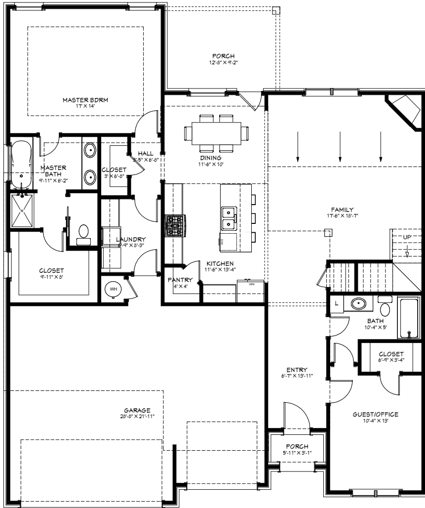
1st Floor
