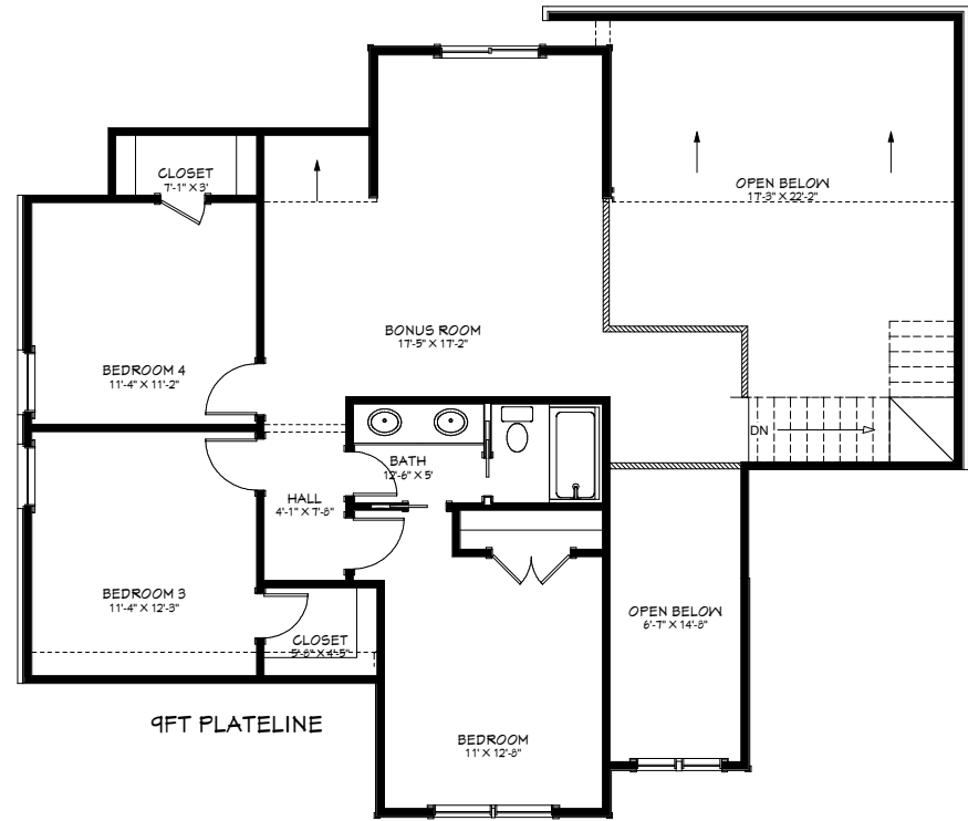
2nd Floor
